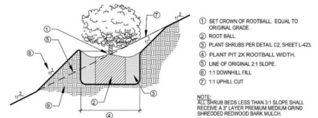
G SLOPE SHRUB PLANTING DETAIL NO SCALE
