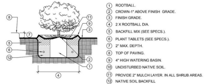
D SHRUB PLANTING DETAIL NO SCALE
